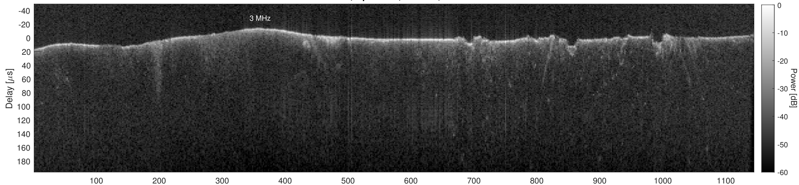
Orbit 13282, Cluttergram
