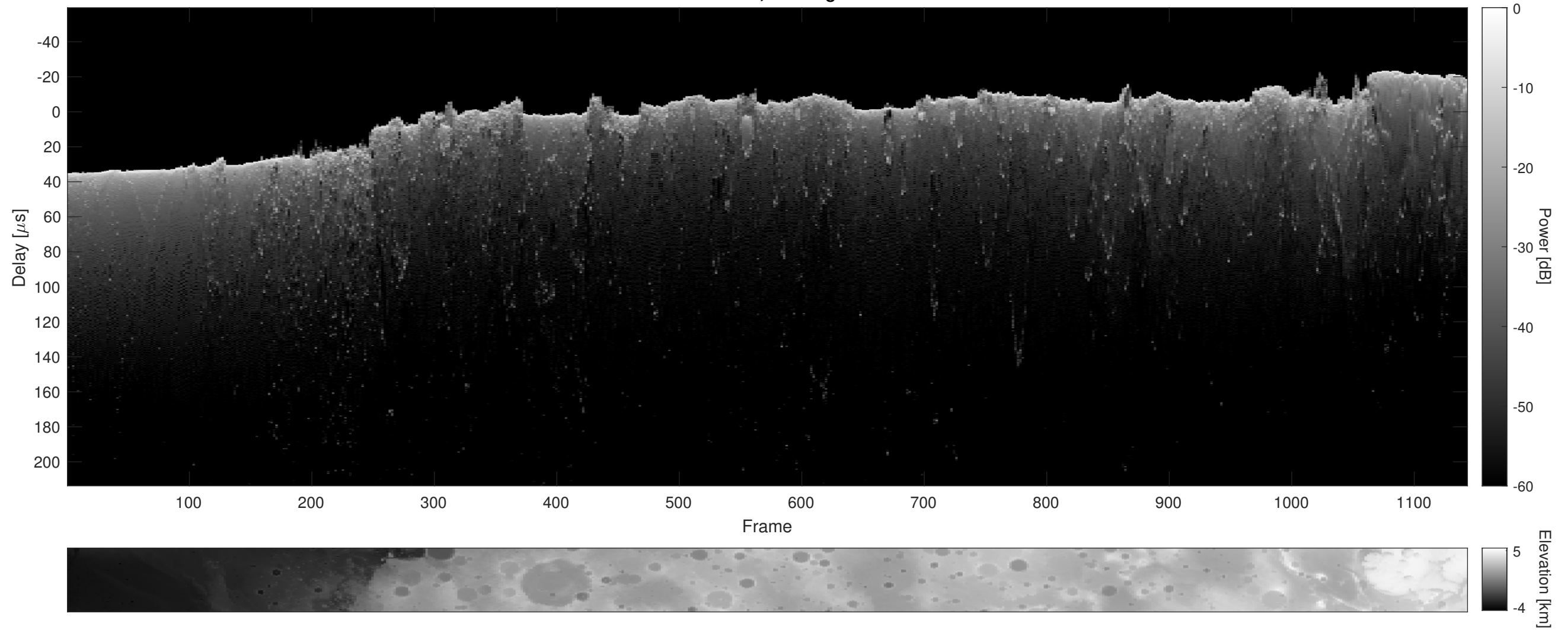
Orbit 13283, Cluttergram
