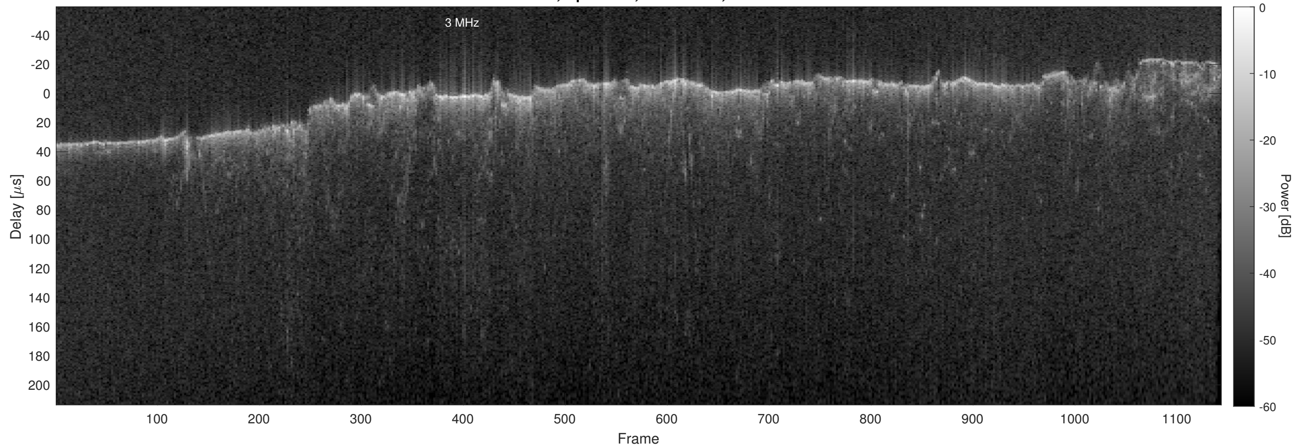
Orbit 13283, Optimized, No Window, Channel 2
