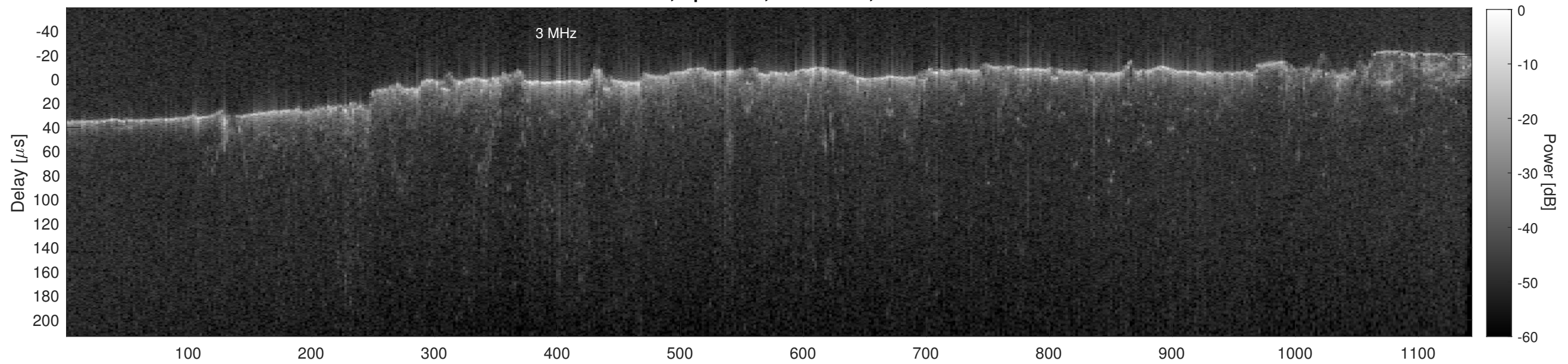
Orbit 13283, Cluttergram
