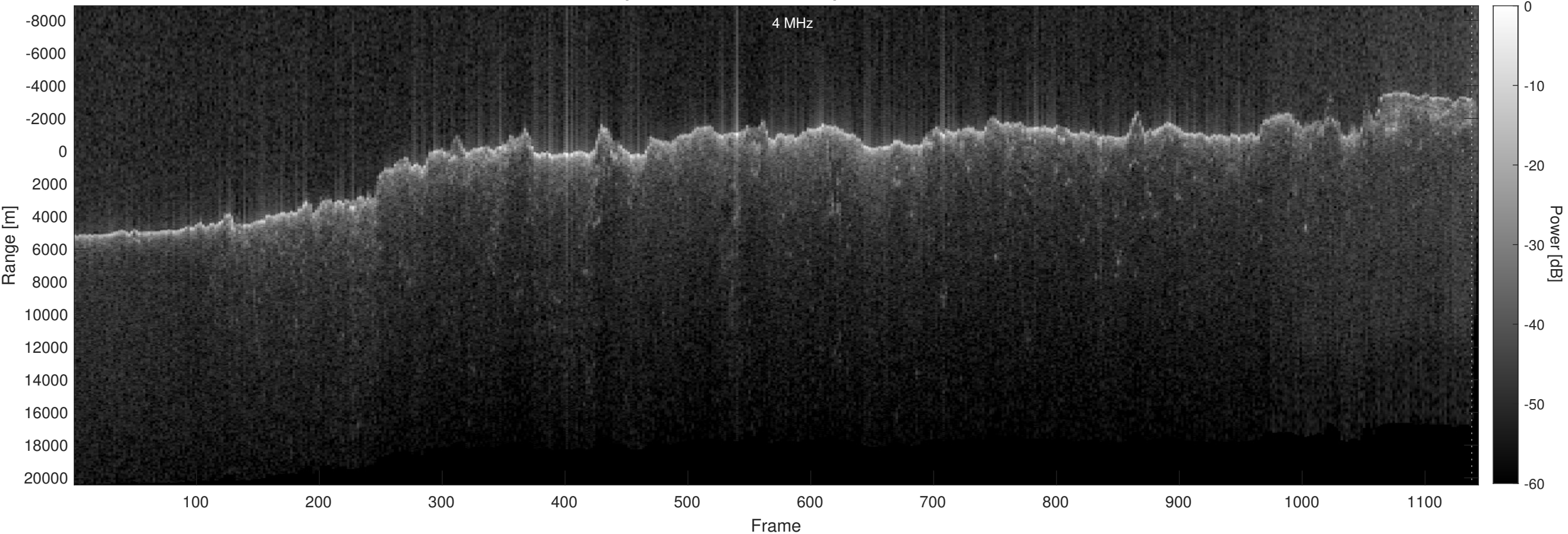
Orbit 13283, Optimized, No Window, Depth-Corrected, Channel 2
