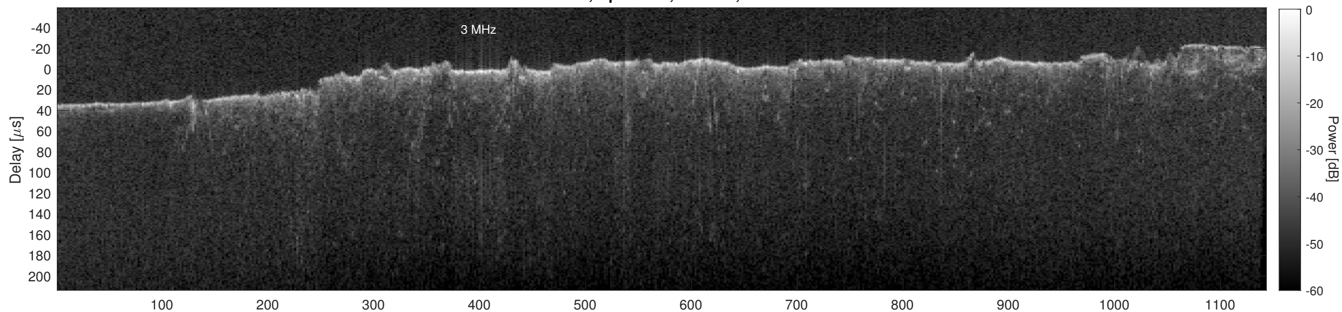
Orbit 13283, Cluttergram
