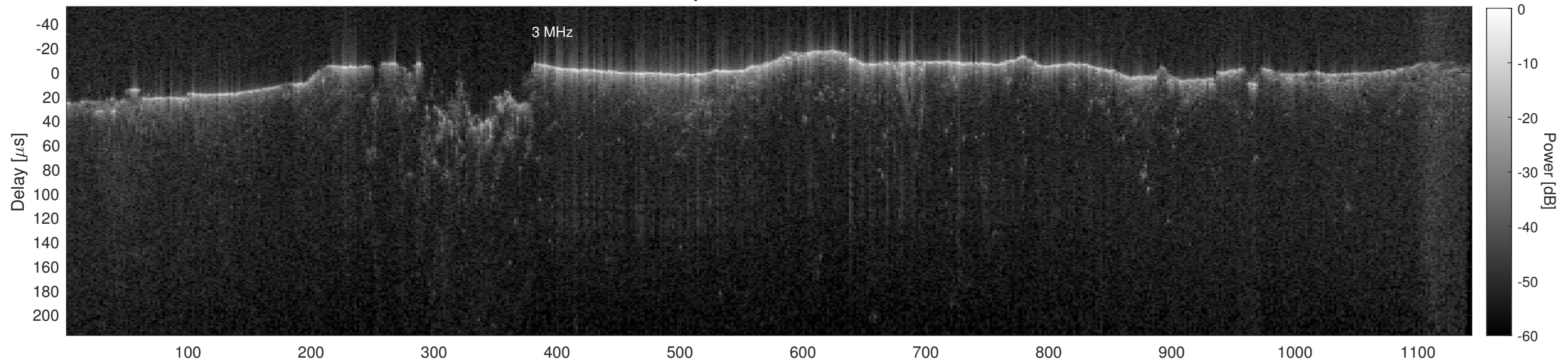
Orbit 13285, Cluttergram
