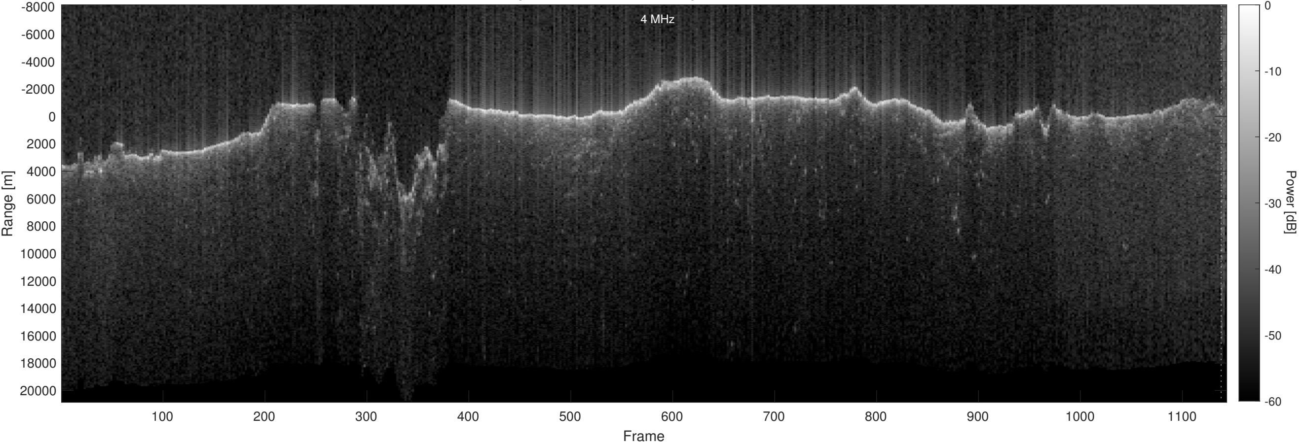
Orbit 13285, Optimized, No Window, Depth-Corrected, Channel 2
