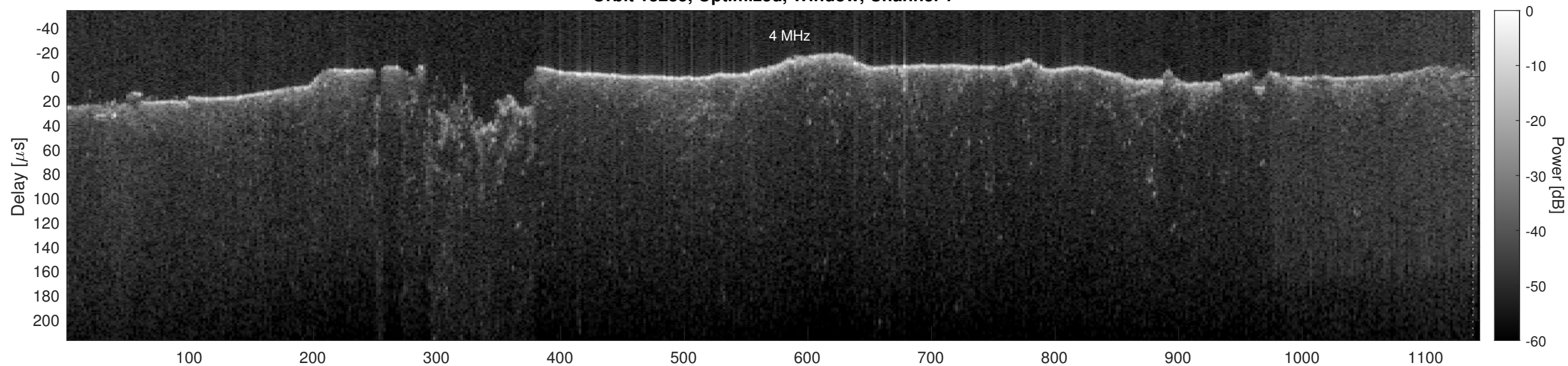
Orbit 13285, Optimized, Window, Channel 2
