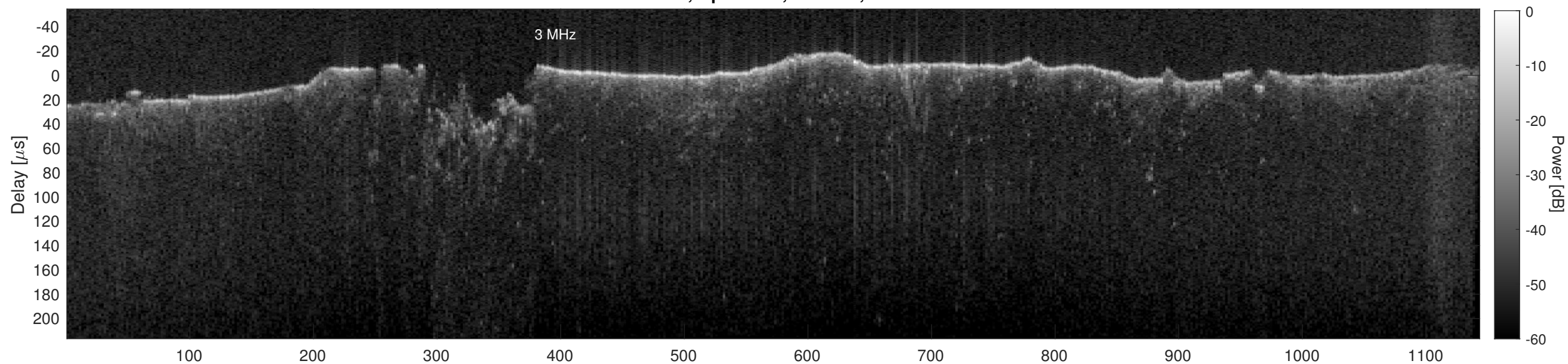
Orbit 13285, Cluttergram
