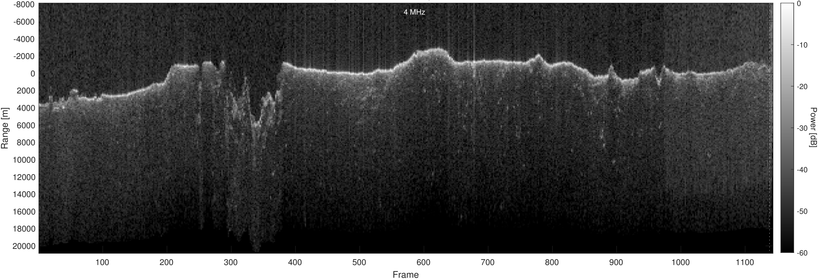
Orbit 13285, Optimized, Window, Depth-Corrected, Channel 2
