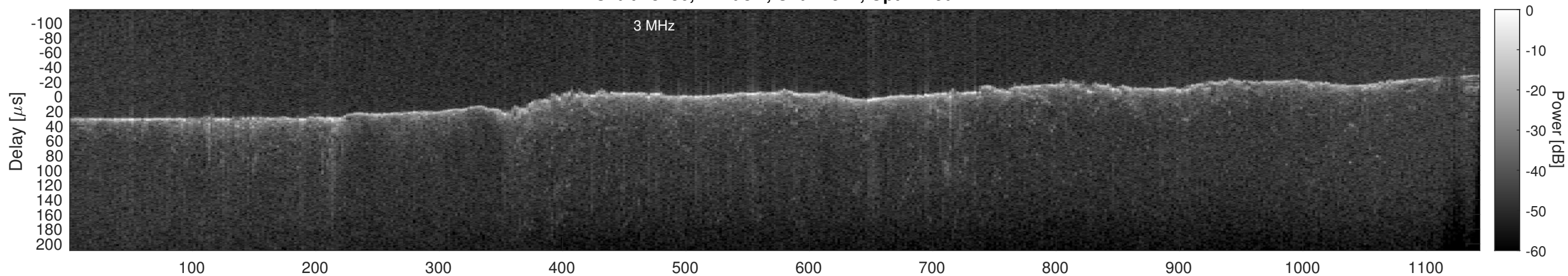
Orbit 13286, Cluttergram
