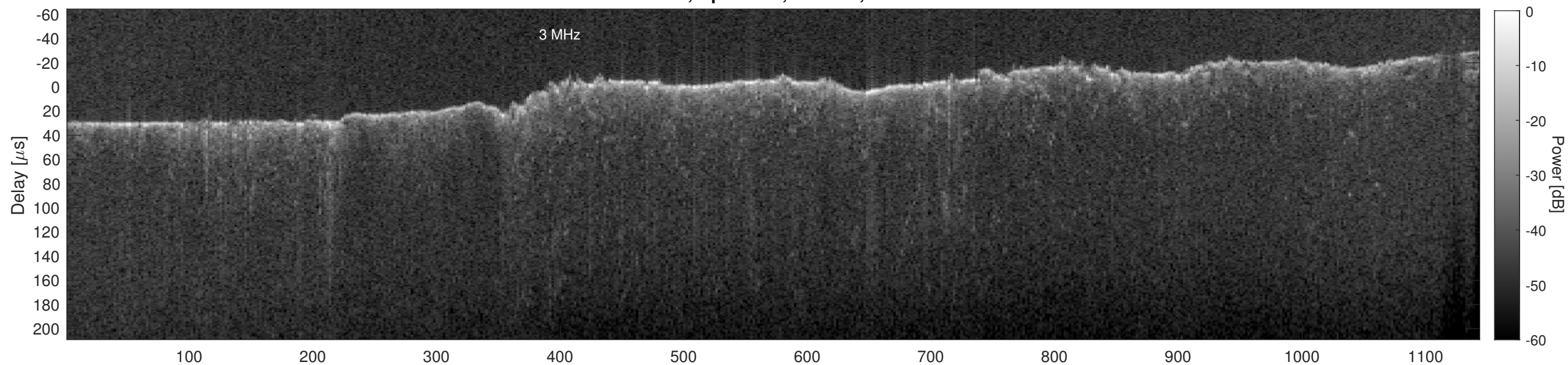
Orbit 13286, Cluttergram
