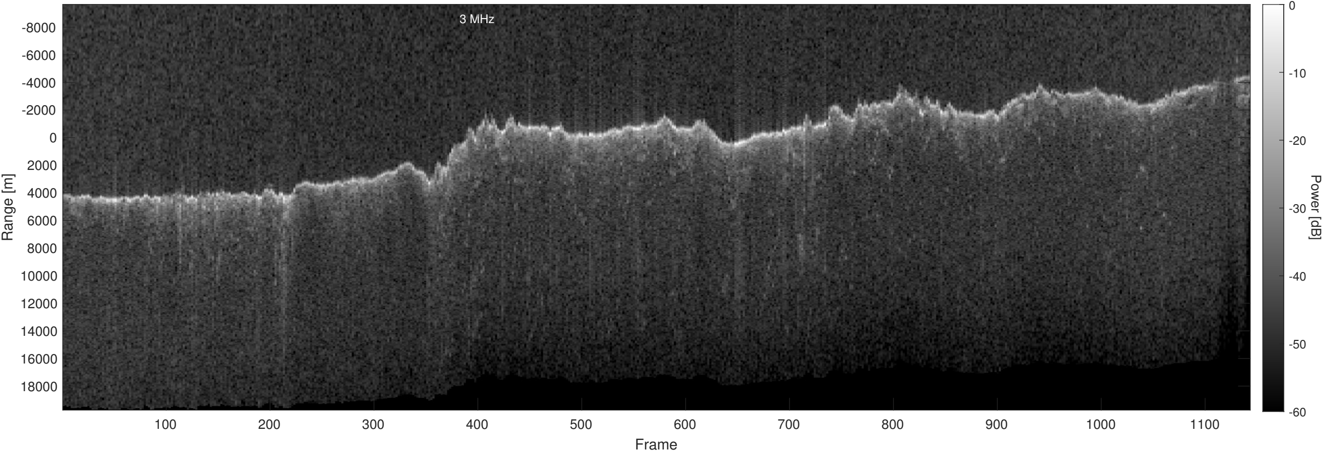
Orbit 13286, Optimized, Window, Depth-Corrected, Channel 2
