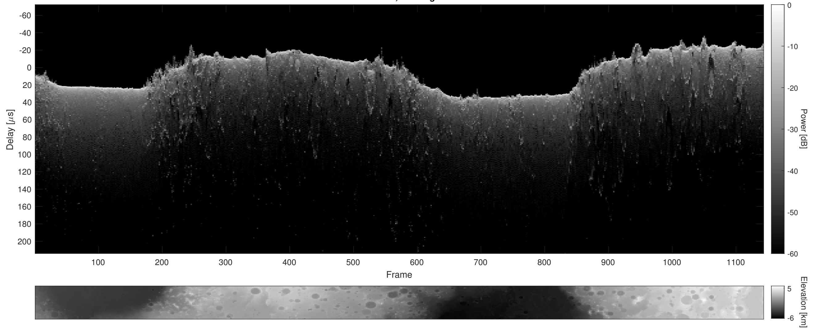
Orbit 13287, Cluttergram
