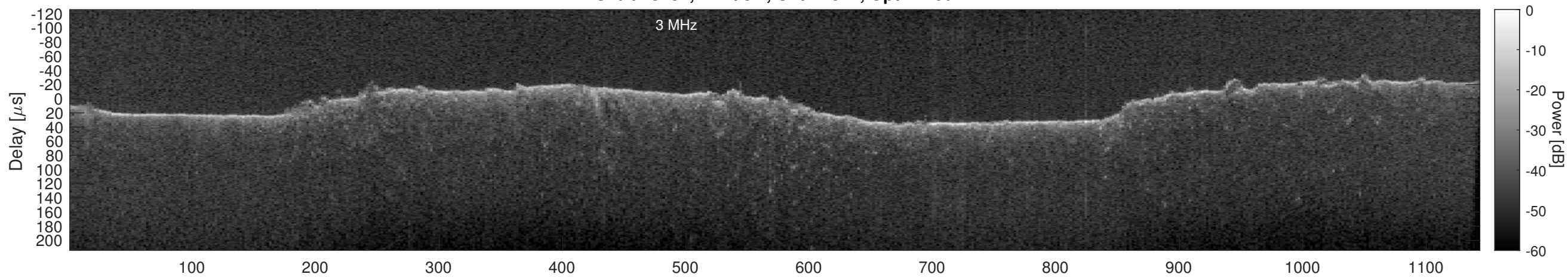
Orbit 13287, Cluttergram
