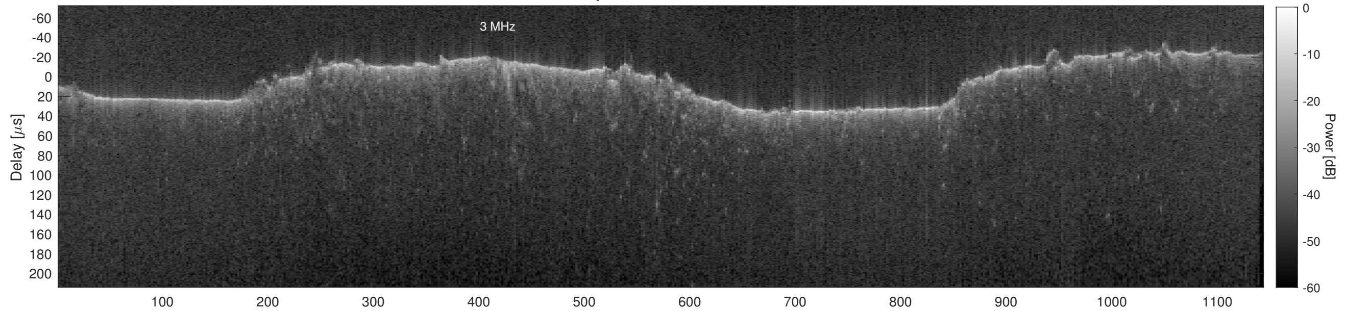
Orbit 13287, Cluttergram
