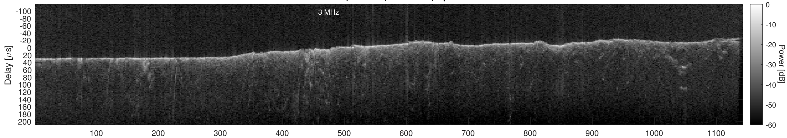
Orbit 13300, Cluttergram
