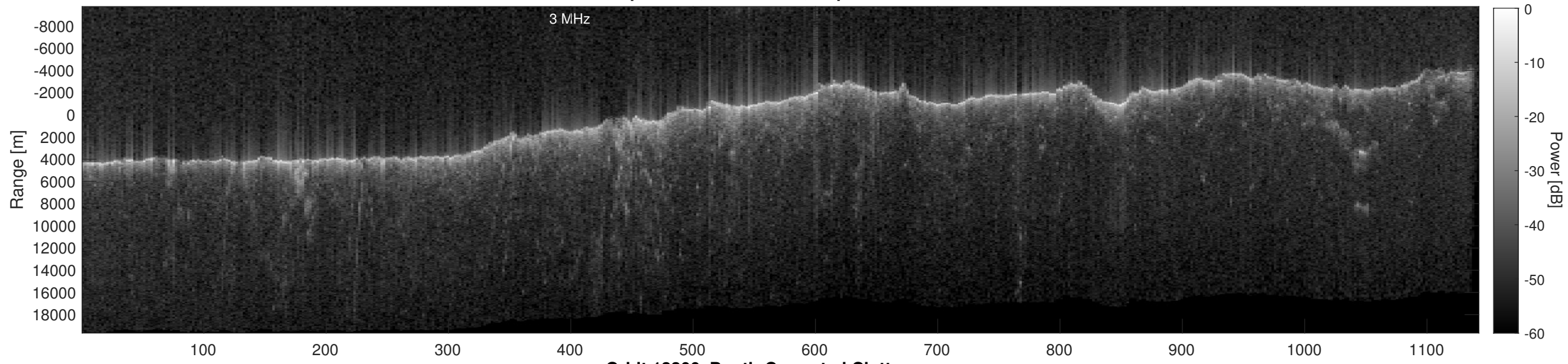
Orbit 13300, Depth-Corrected Cluttergram
