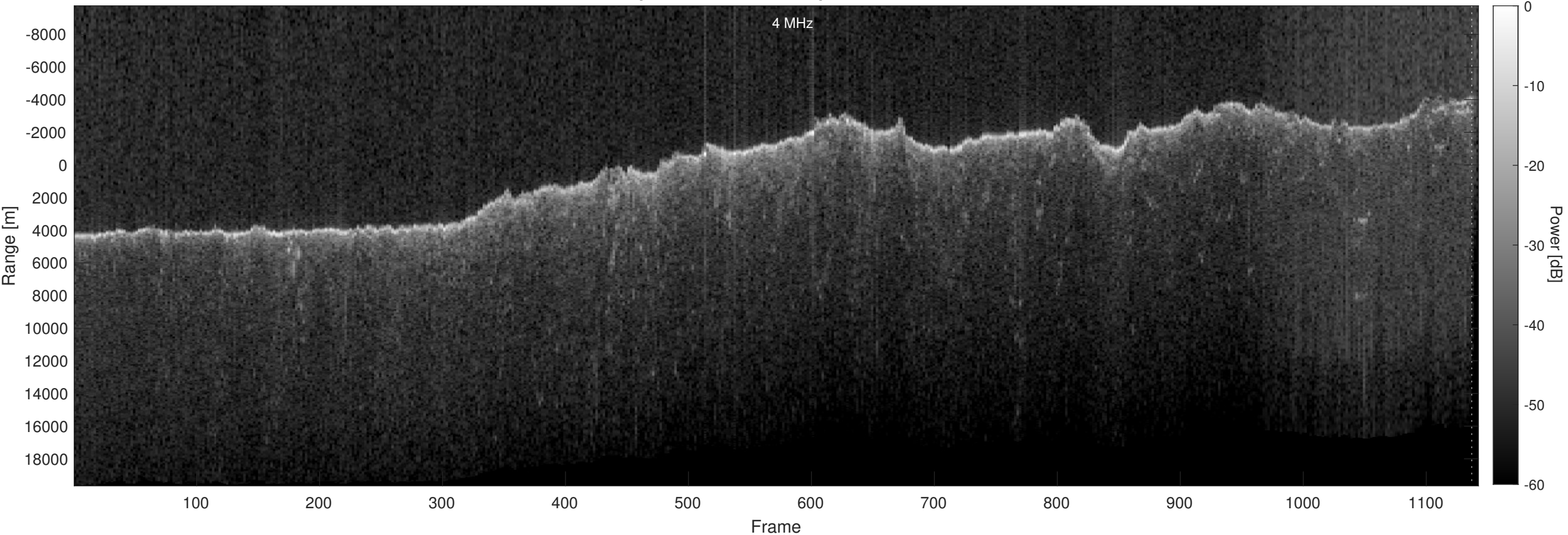
Orbit 13300, Optimized, Window, Depth-Corrected, Channel 2
