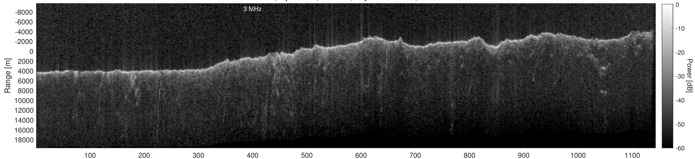
Orbit 13300, Depth-Corrected Cluttergram
