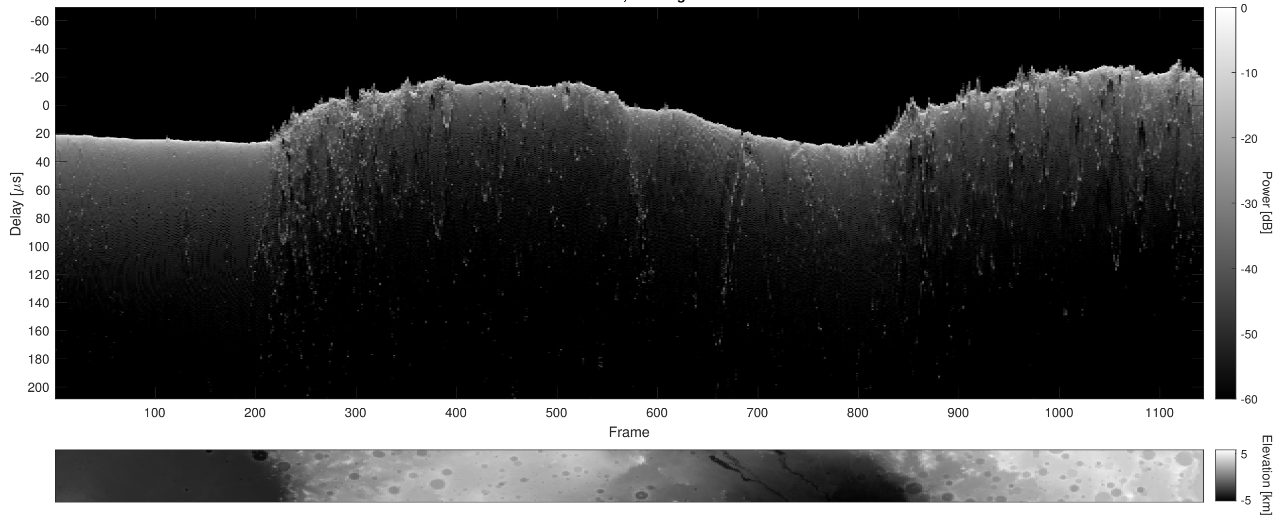
Orbit 13301, Cluttergram
