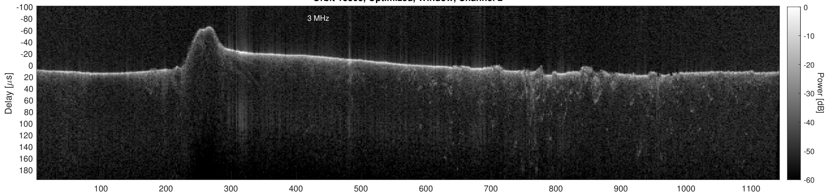
Orbit 13303, Cluttergram
