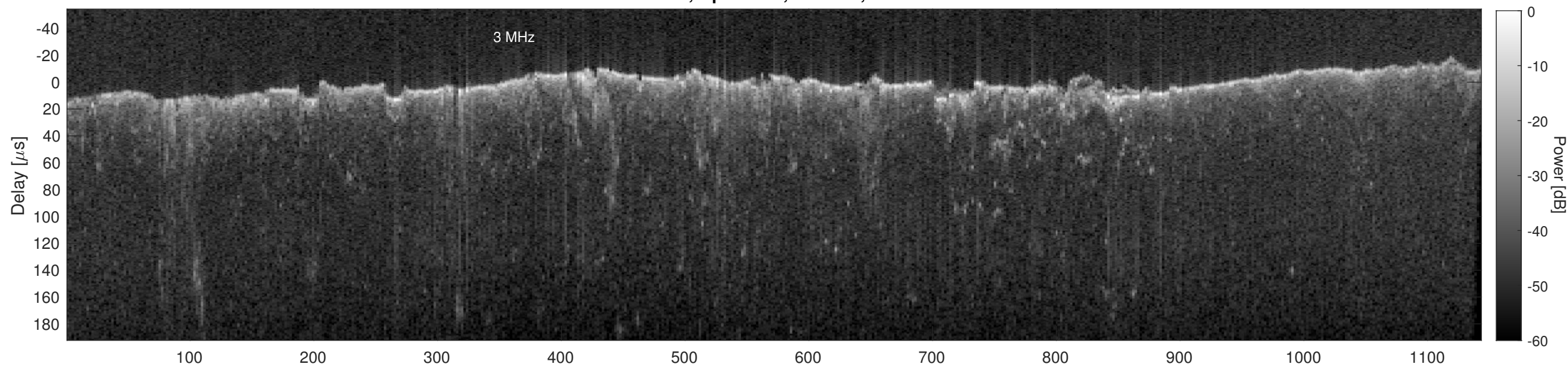
Orbit 13305, Cluttergram
