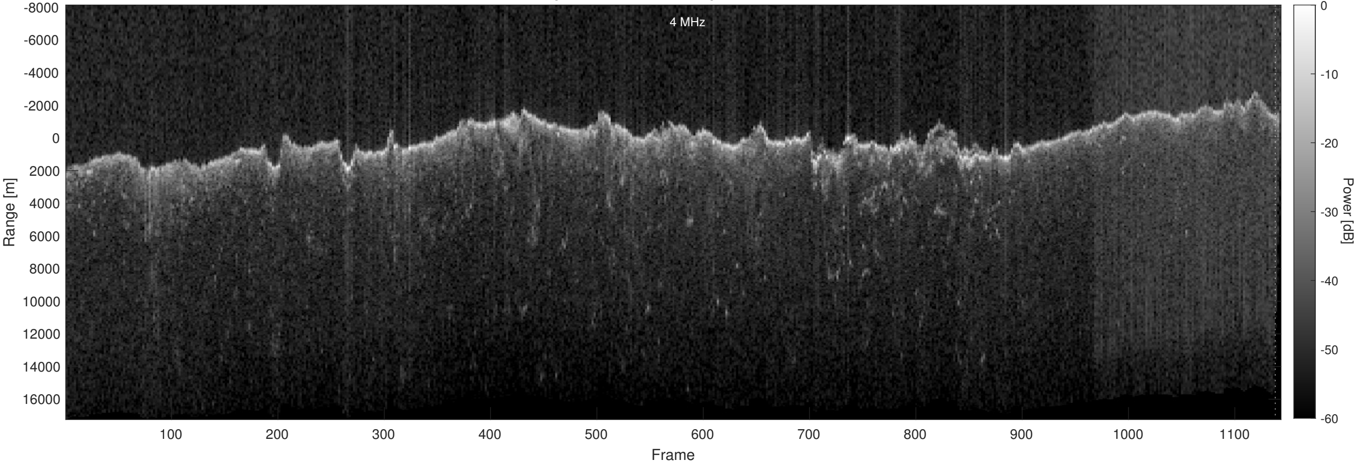
Orbit 13305, Optimized, Window, Depth-Corrected, Channel 2
