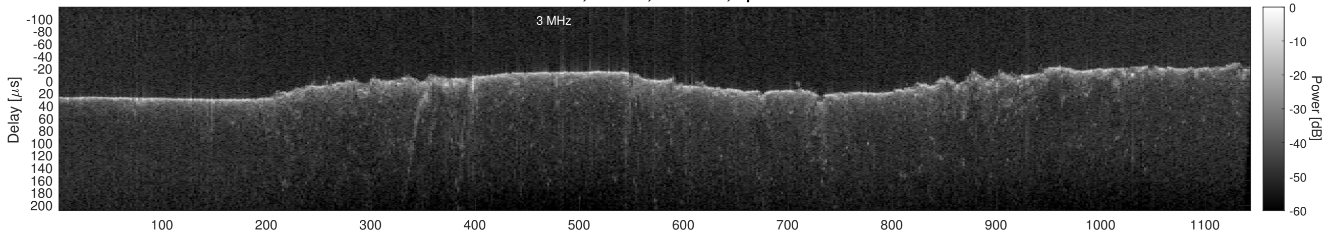
Orbit 13308, Cluttergram
