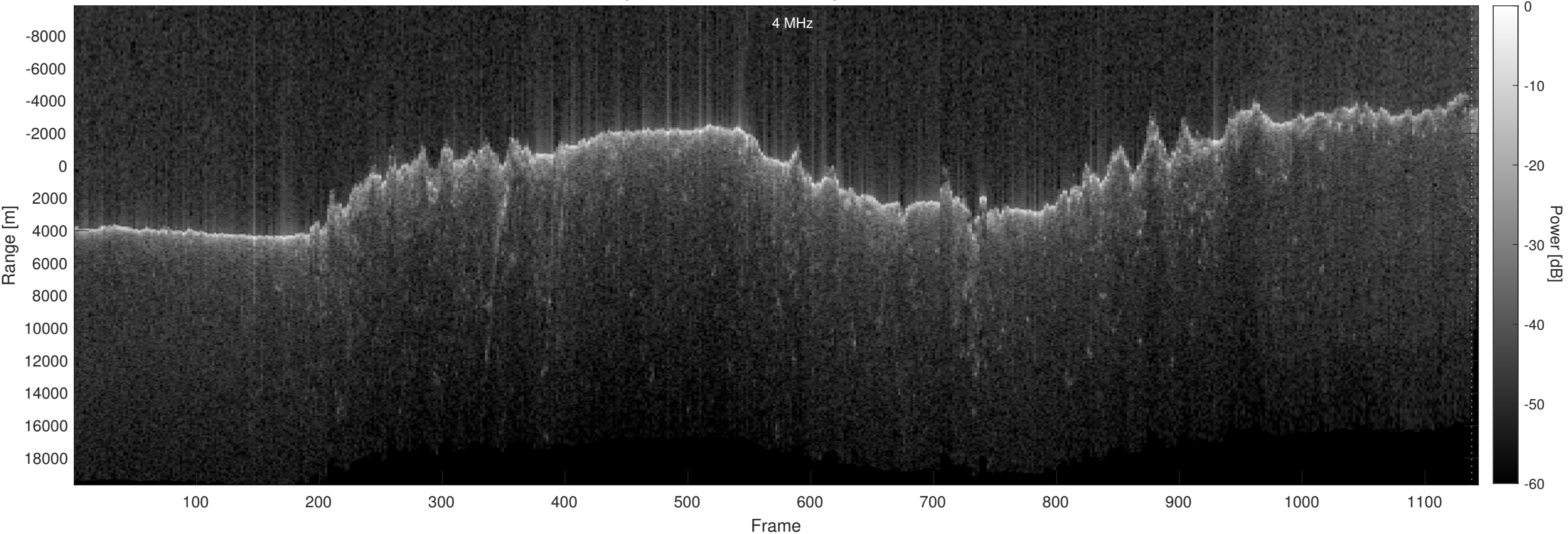
Orbit 13308, Optimized, No Window, Depth-Corrected, Channel 2
