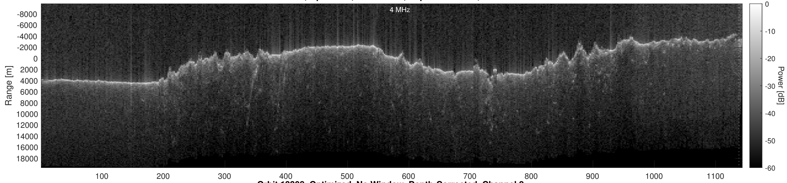
Orbit 13308, Optimized, No Window, Depth-Corrected, Channel 2
