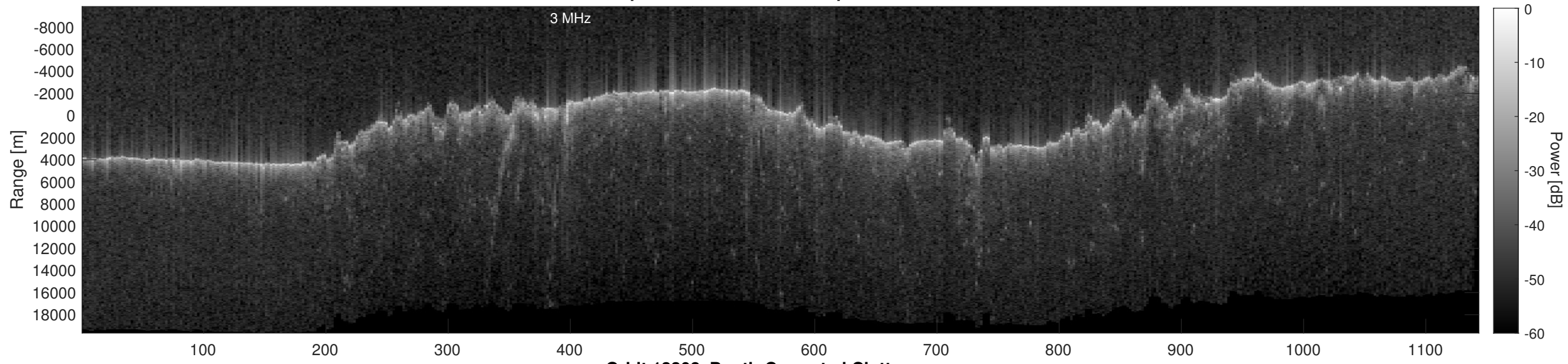
Orbit 13308, Depth-Corrected Cluttergram
