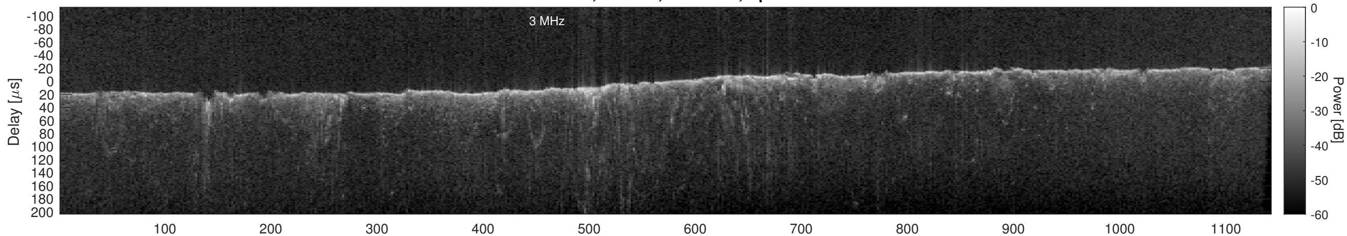
Orbit 13309, Cluttergram
