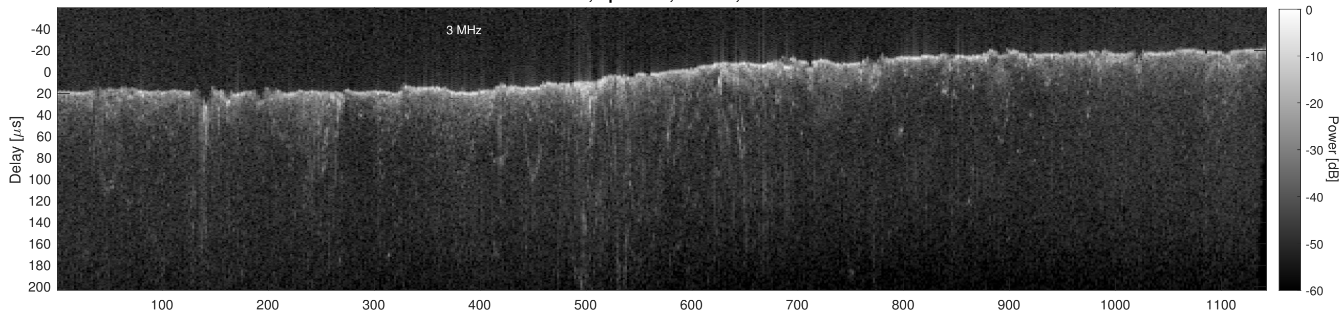
Orbit 13309, Cluttergram
