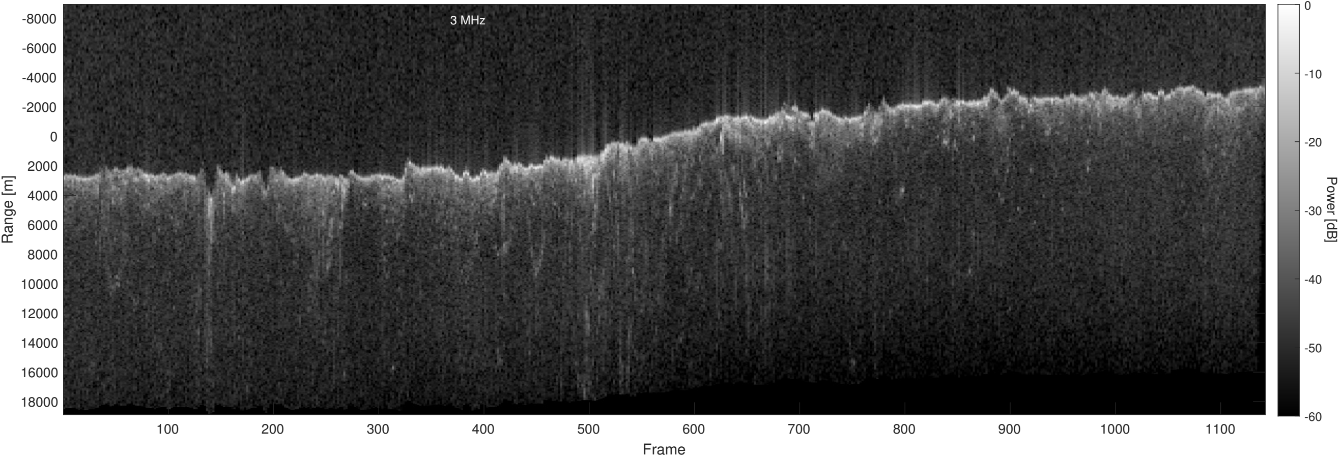
Orbit 13309, Optimized, Window, Depth-Corrected, Channel 2
