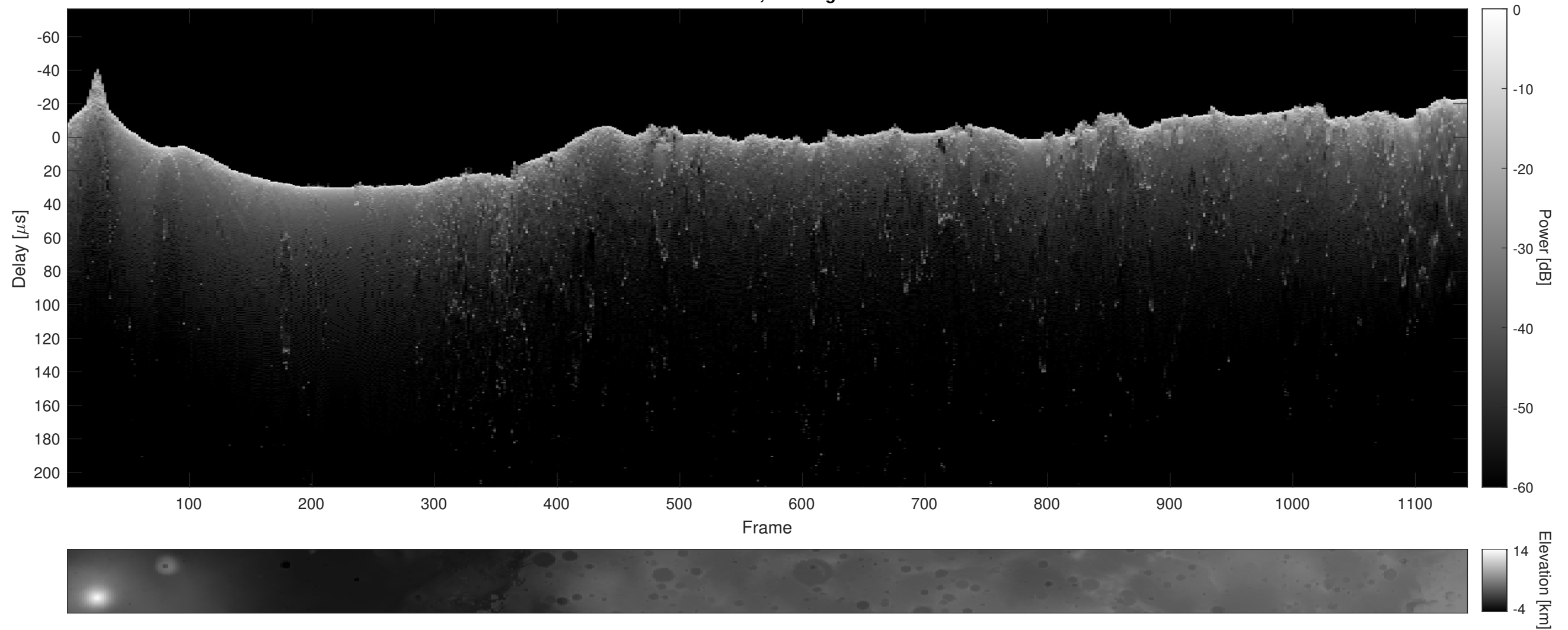
Orbit 13311, Cluttergram
