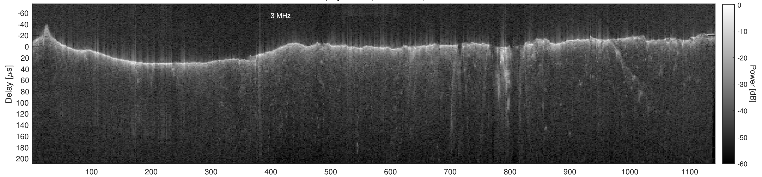
Orbit 13311, Cluttergram
