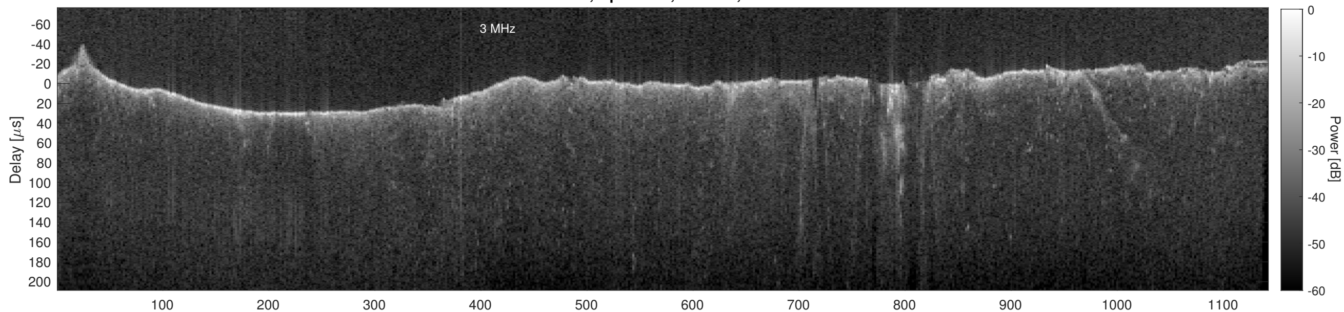
Orbit 13311, Cluttergram
