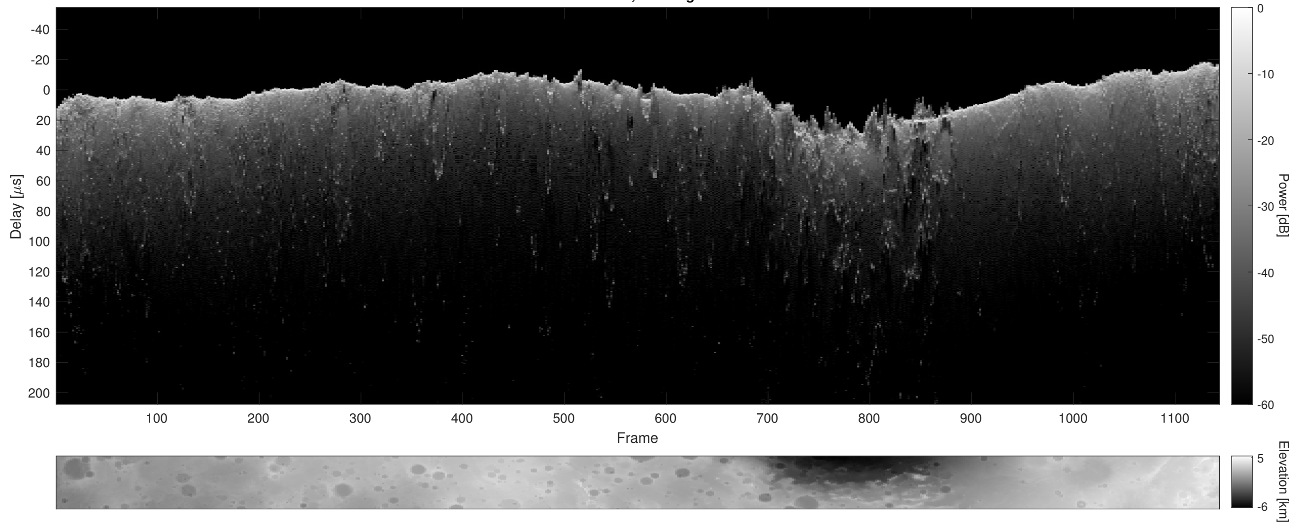
Orbit 13312, Cluttergram
