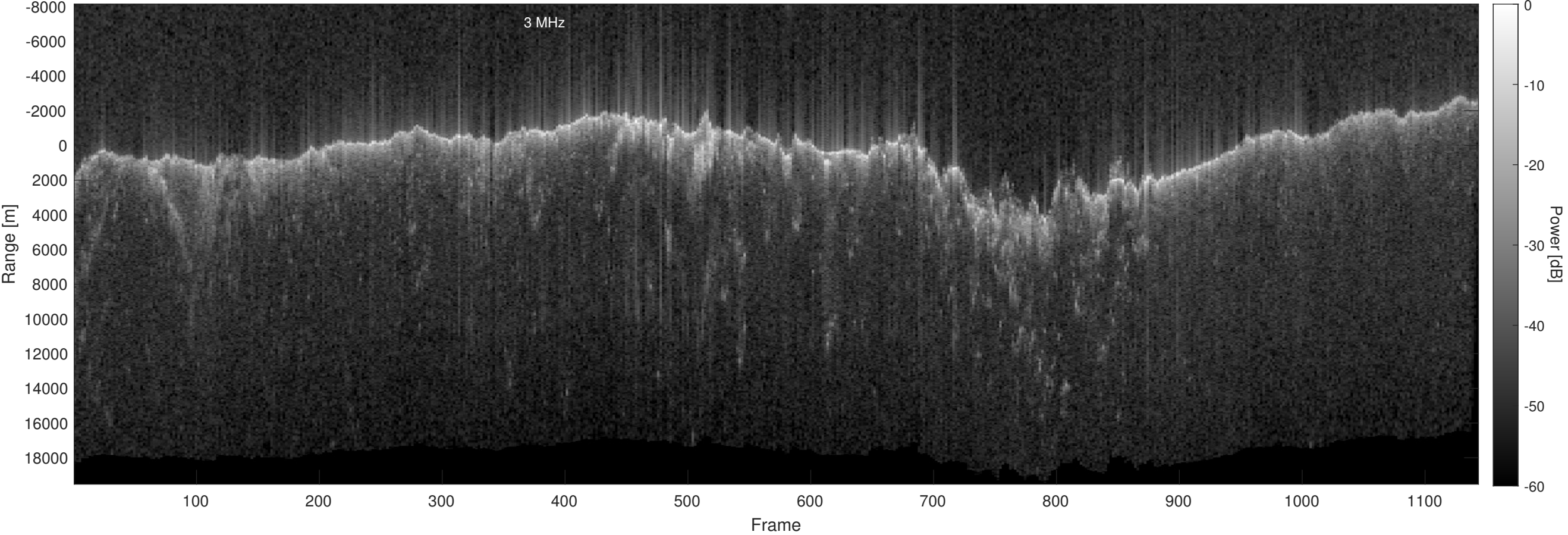
Orbit 13312, Optimized, No Window, Depth-Corrected, Channel 2
