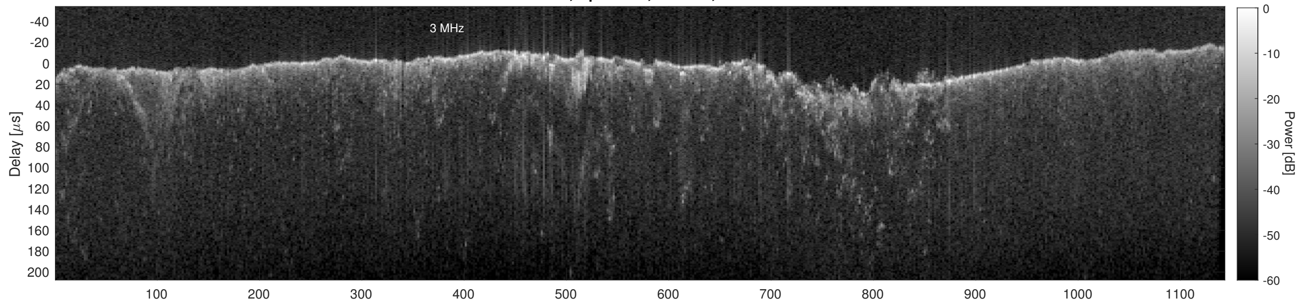
Orbit 13312, Cluttergram
