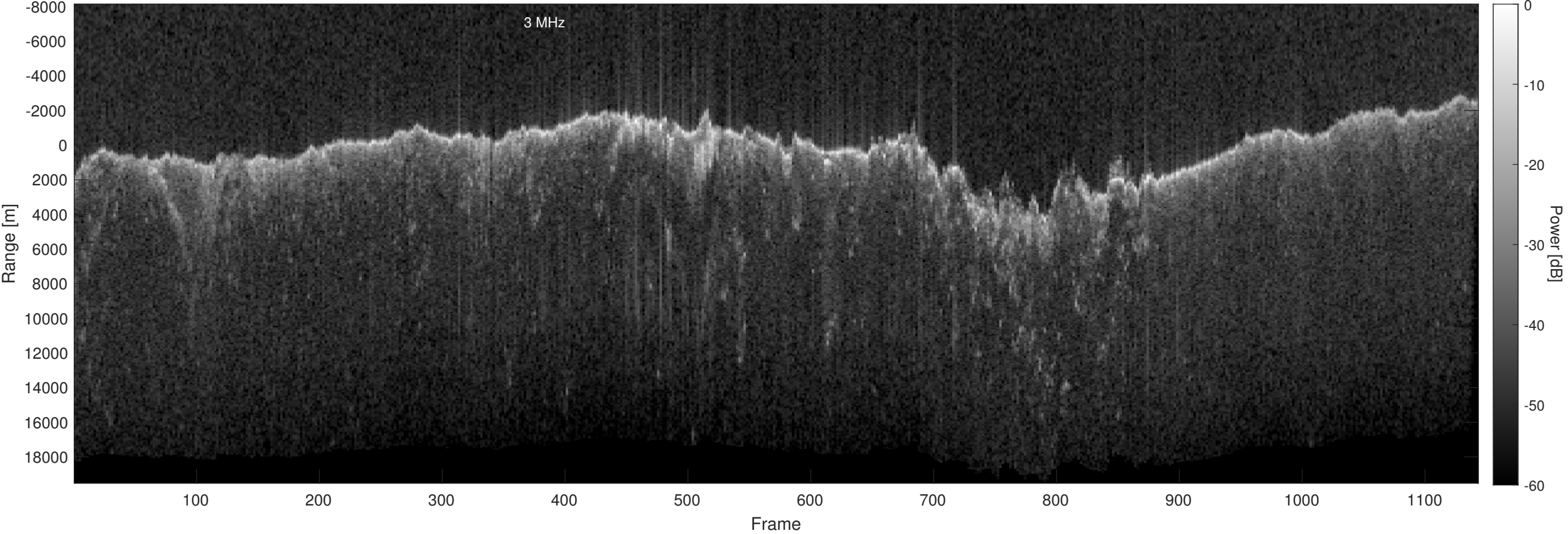
Orbit 13312, Optimized, Window, Depth-Corrected, Channel 2
