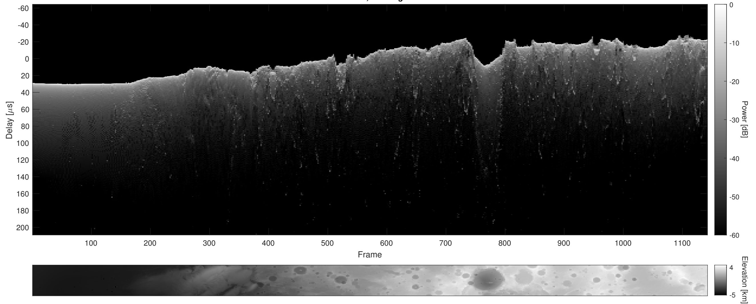
Orbit 13314, Cluttergram
