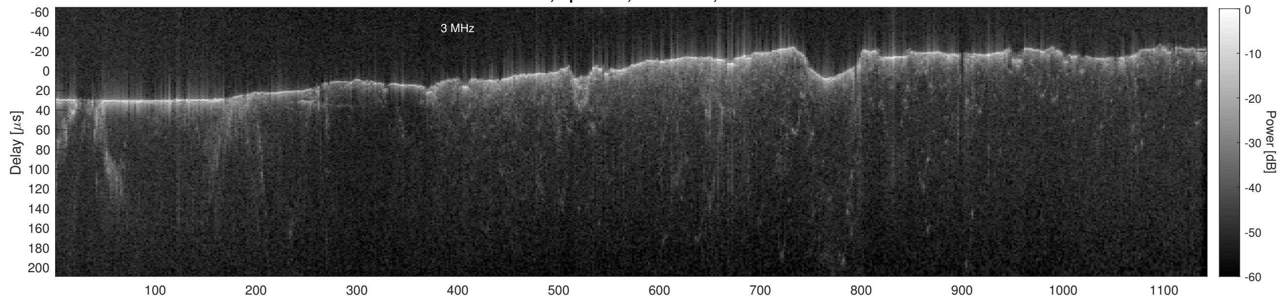
Orbit 13314, Cluttergram
