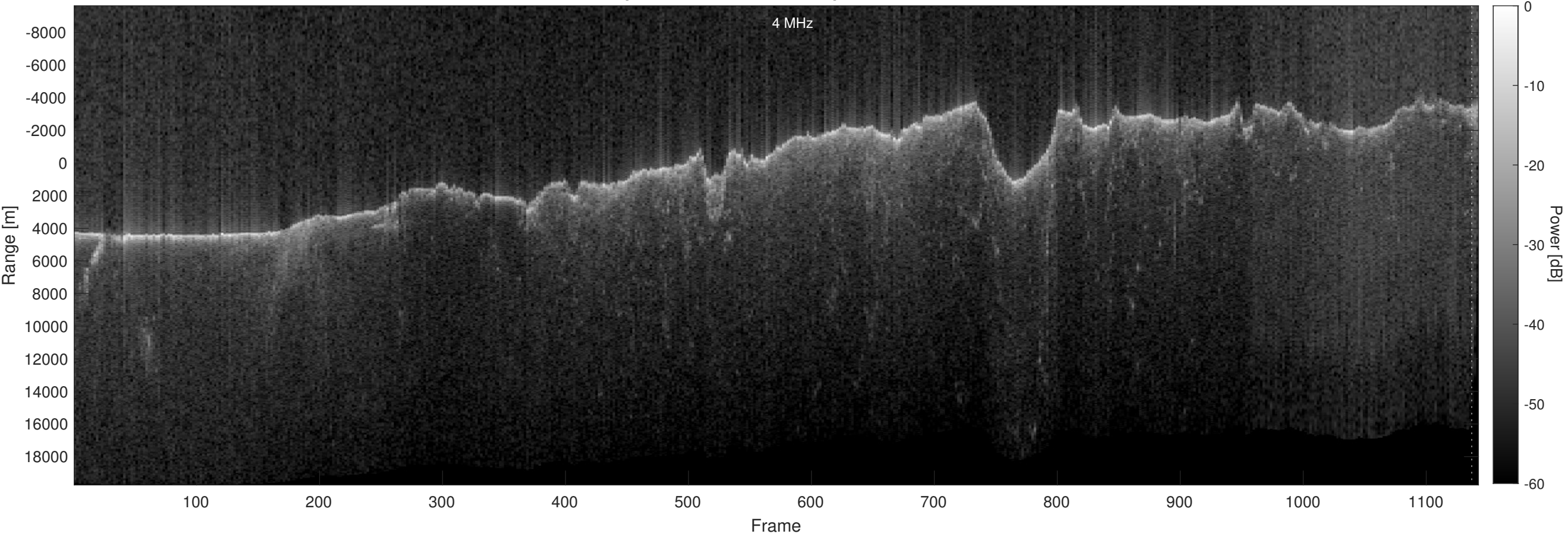
Orbit 13314, Optimized, No Window, Depth-Corrected, Channel 2
