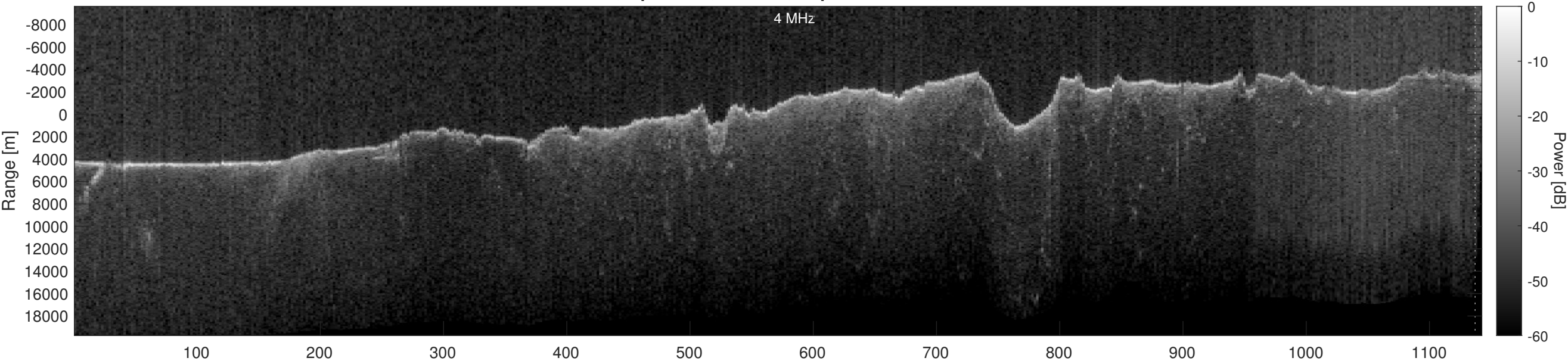
Orbit 13314, Optimized, Window, Depth-Corrected, Channel 2
