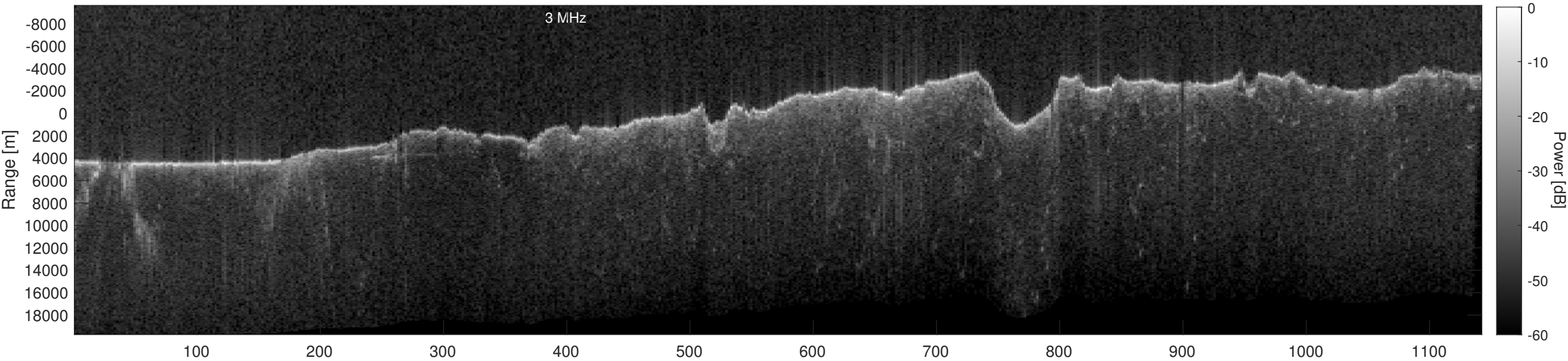
Orbit 13314, Depth-Corrected Cluttergram
