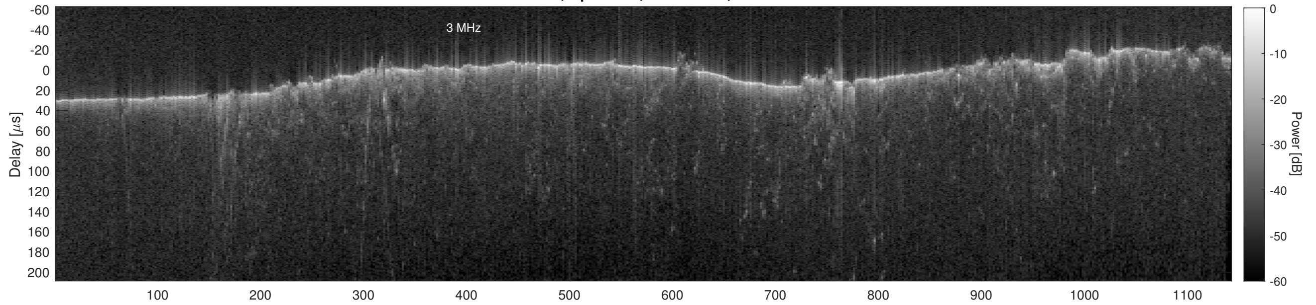
Orbit 13315, Cluttergram
