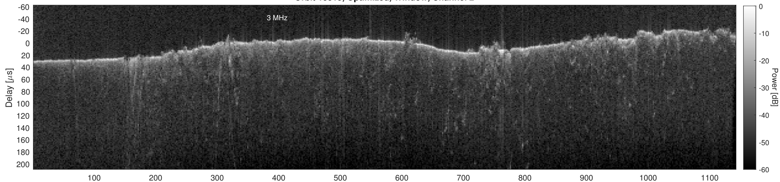
Orbit 13315, Cluttergram
