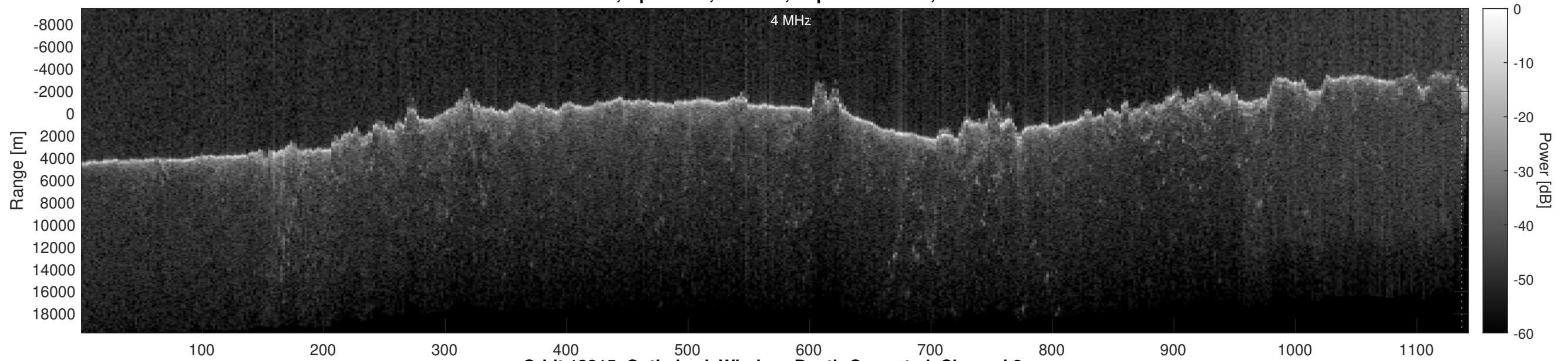
Orbit 13315, Optimized, Window, Depth-Corrected, Channel 2
