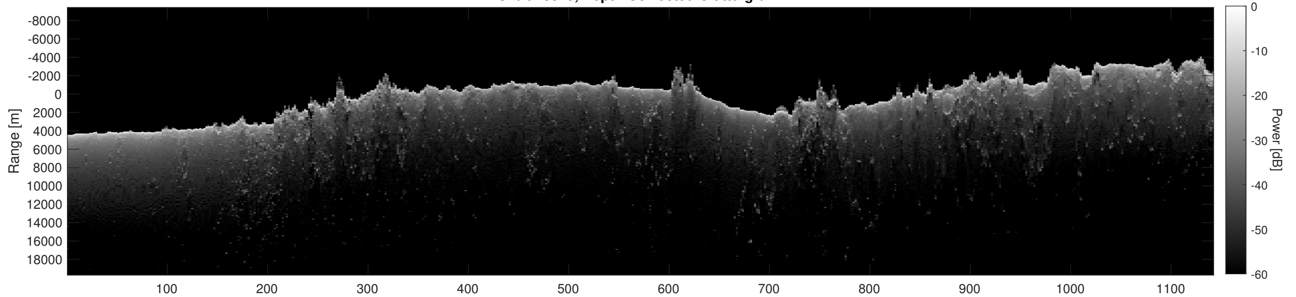
Orbit 13315, Depth-Corrected Cluttergram
