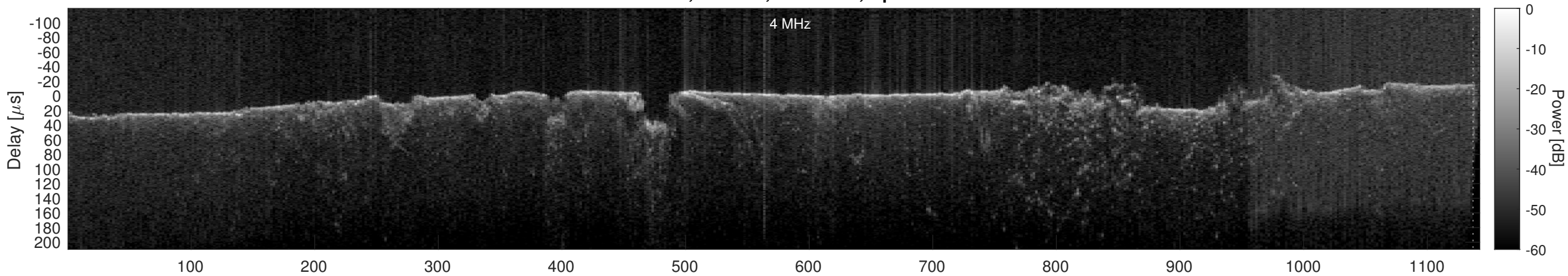
Orbit 13320, Cluttergram
