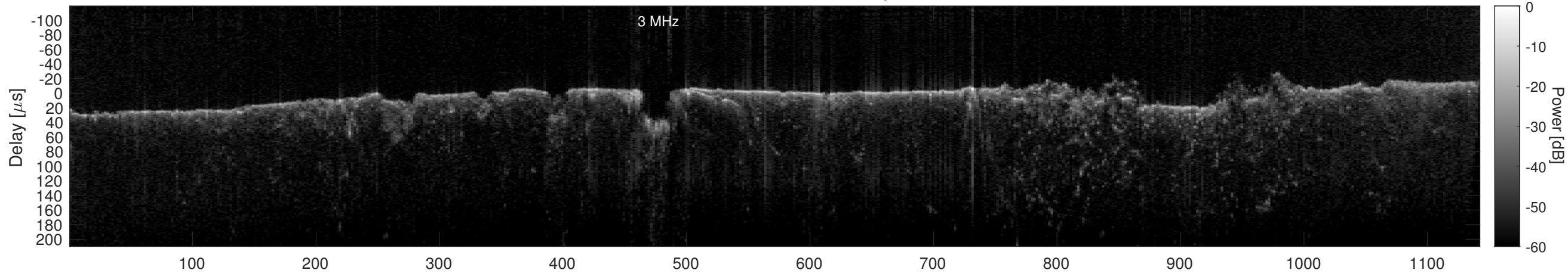
Orbit 13320, Cluttergram
