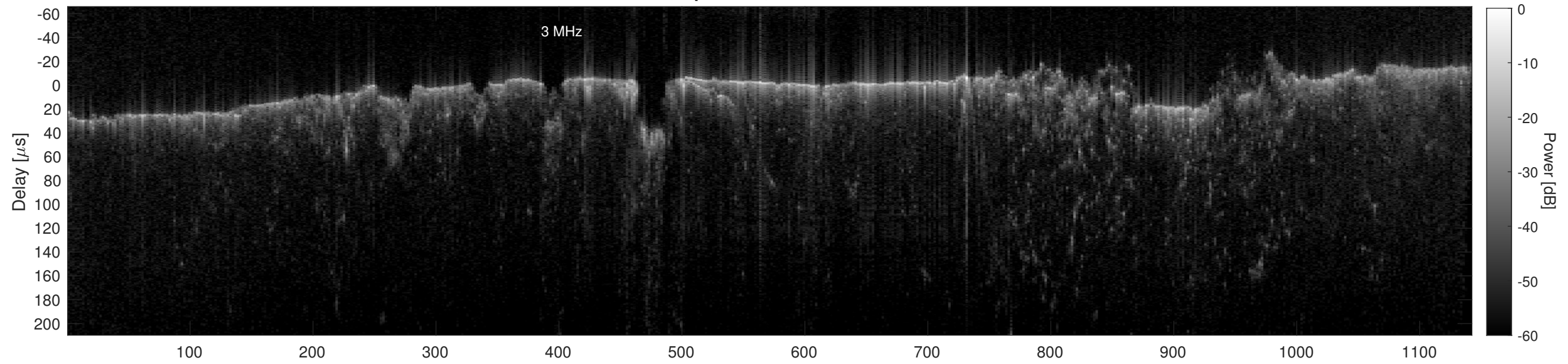
Orbit 13320, Cluttergram
