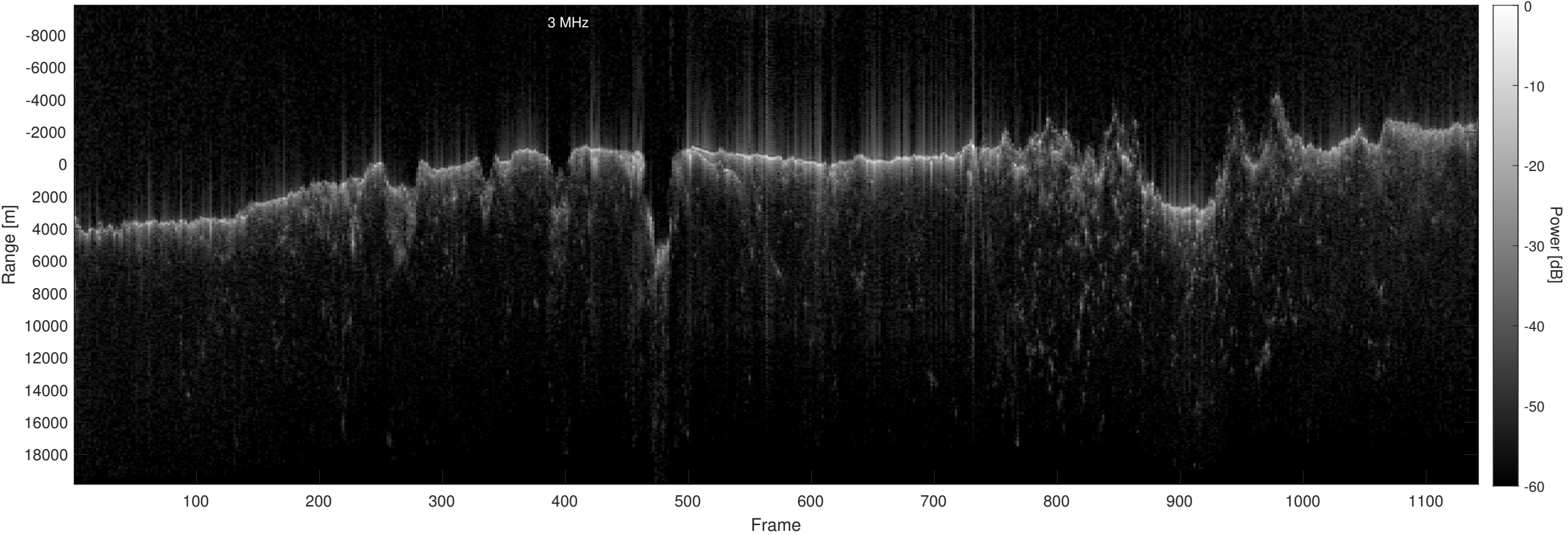
Orbit 13320, Optimized, No Window, Depth-Corrected, Channel 2
