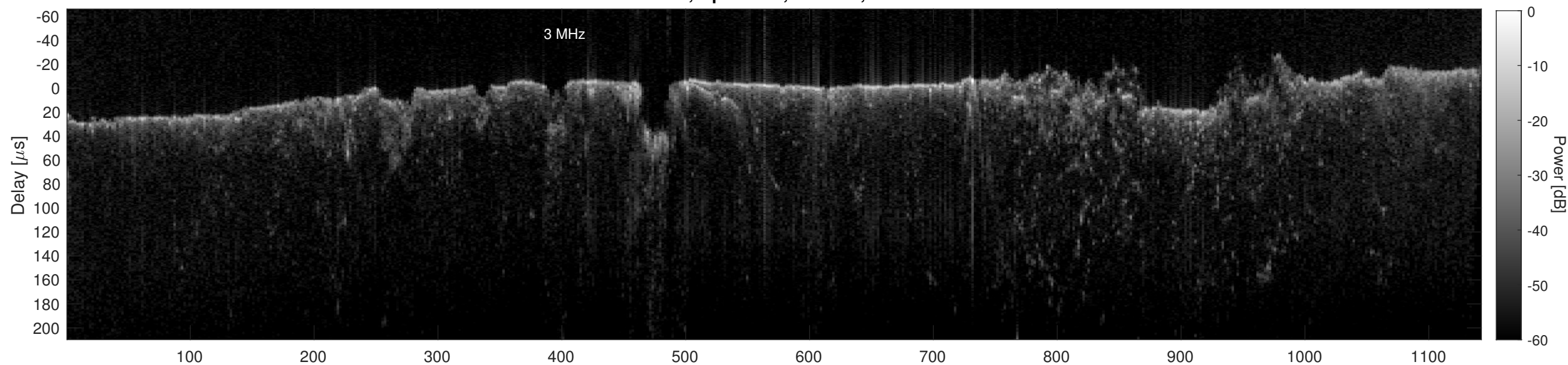
Orbit 13320, Cluttergram
