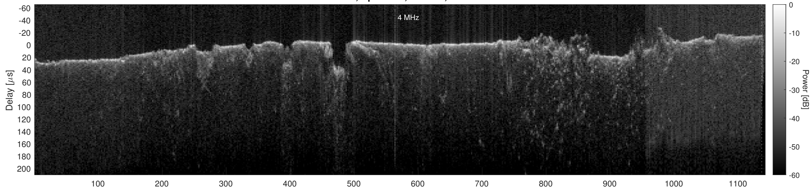
Orbit 13320, Optimized, Window, Channel 2
