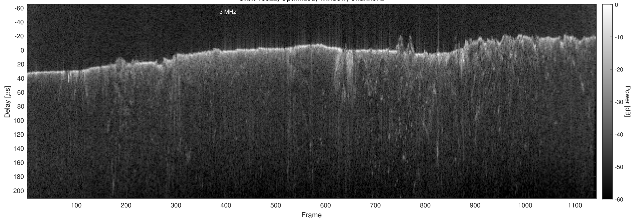
Orbit 13322, Optimized, Window, Channel 2
